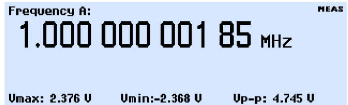
Multi-parameter Display.
